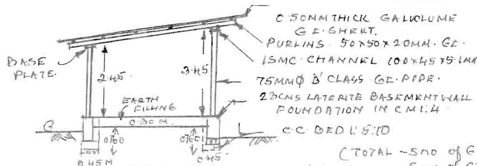
CROSS SECTION A.B.
