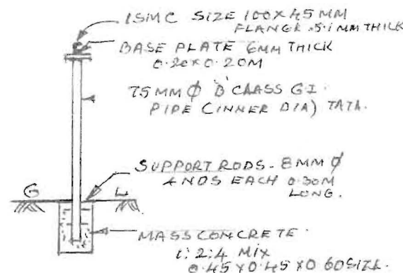
SECTION OF G.I. PIPE.
