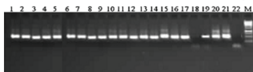
Fig. 3 Detection of RWD phytoplasma with semi-nested PCR IF7/7R3-IF7/7R2. Lanes 1-5: samples from Kasaragod. Lanes 6-20: samples from Kayamkulam. Lane 21: positive control (sugarcane grassy shoot). Lane 22: asymptomatic palm from Kayamkulam. Lane M: 1-kb ladder
