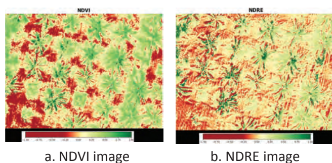
Fig. 23. Multispectral images captured using drone and converted to NDVI and NDRE images; a) NDVI image – index used for leaf coverage and plant health; b) NDRE image : Index sensitive to content of leaves against soil background
