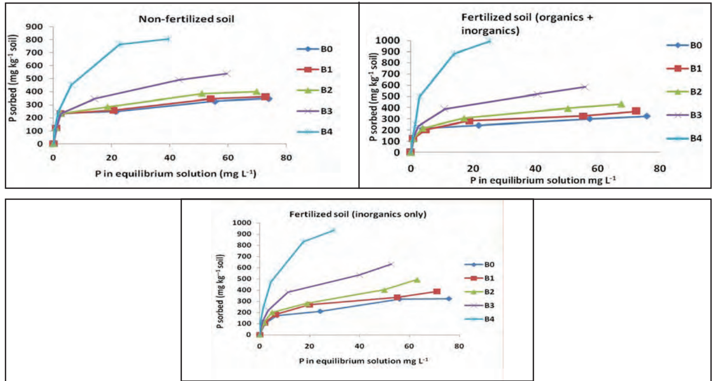
Fig. 15. Phosphorous profiles in different soil treatment.
